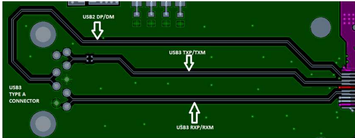
图 59. Example Routing of Downstream Port
