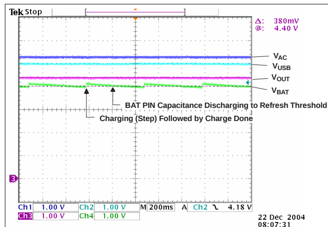
Figure 14. Battery Absent – PWR XFER to USB
