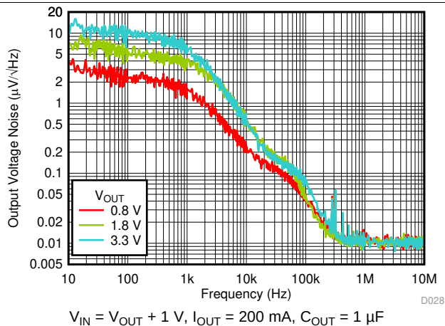
图 45. Output Noise vs Frequency and V_{OUT}
