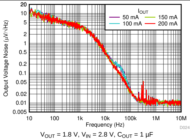
图 43. Output Noise vs Frequency and I_{OUT}
