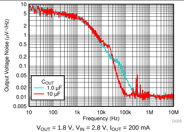
图 44. Output Noise vs Frequency and C_{OUT}
