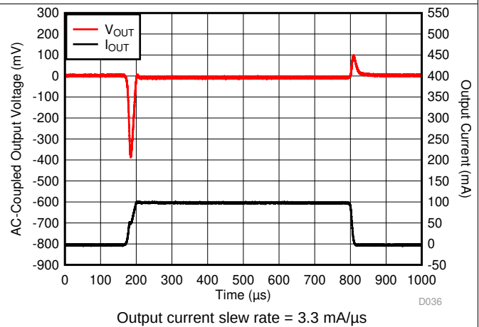
图 6. I_{OUT} Transient 0 mA to 100 mA
