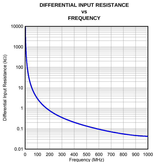
Figure 52. ADC Analog Input Resistance ( R_{in} ) Across Frequency
