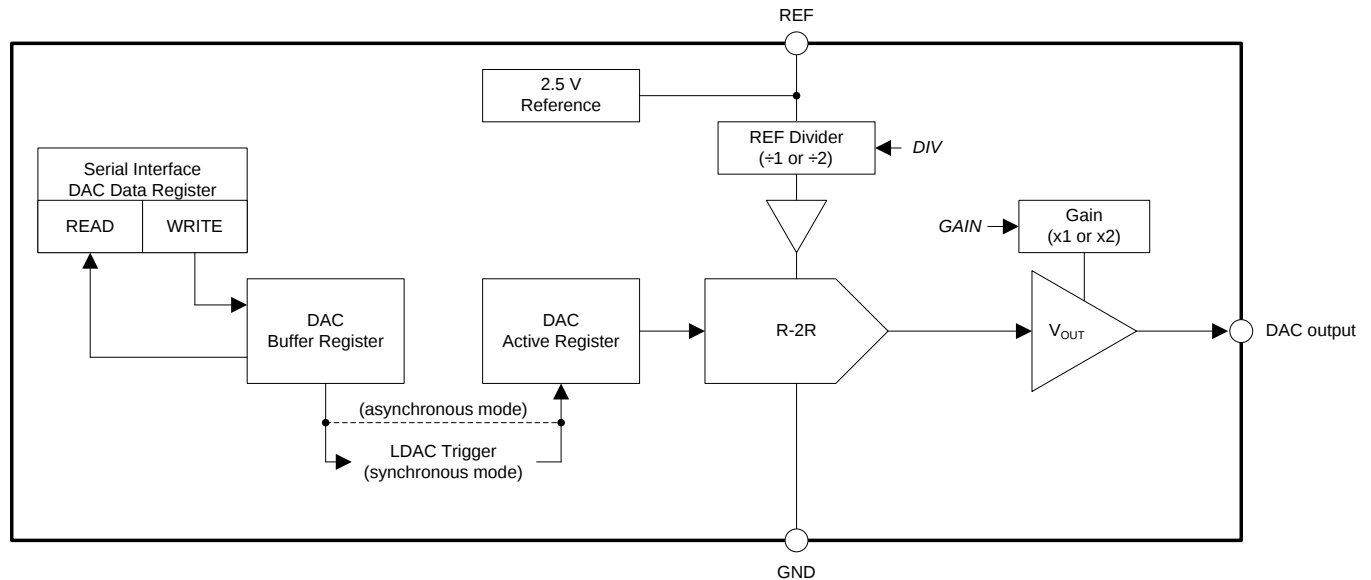
Figure 59. DACx0508 DAC Block Diagram
