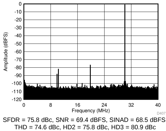
Figure 67. FFT for 270-MHz Input Signal (Dither On)
