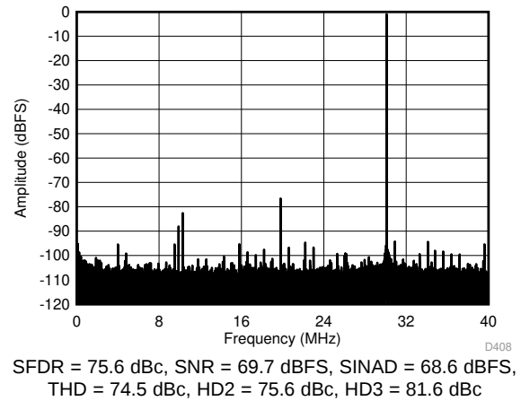
Figure 68. FFT for 270-MHz Input Signal (Dither Off)
