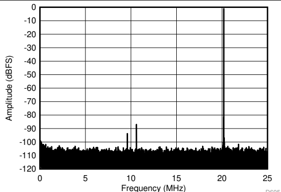
Figure 33. FFT for 70-MHz Input Signal (Dither On)
