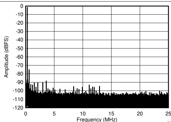
Figure 38. FFT for 270-MHz Input Signal (Dither Off)
