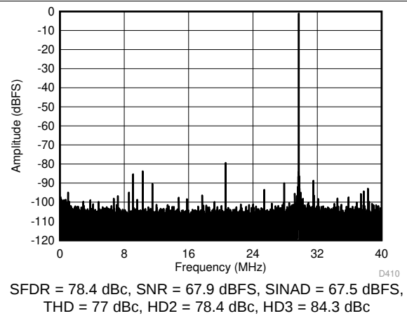
Figure 70. FFT for 450-MHz Input Signal (Dither Off)
