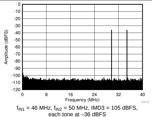
Figure 72. FFT for Two-Tone Input Signal ( -36\text{ dBFS} at 46 MHz and 50 MHz)
