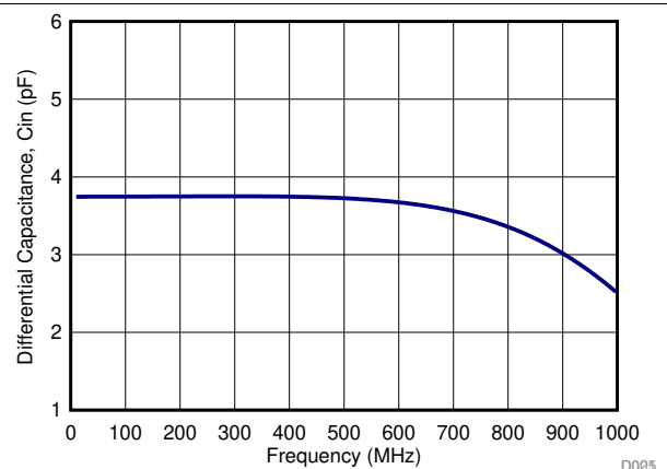
Figure 174. Differential Input Capacitance (C IN )
