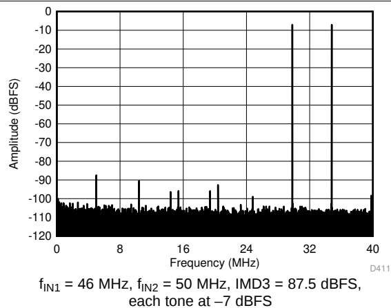
Figure 71. FFT for Two-Tone Input Signal ( -7\text{ dBFS} at 46 MHz and 50 MHz)
