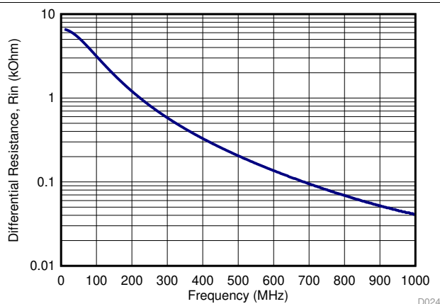
Figure 173. Differential Input Resistance (R IN )
