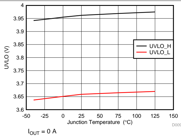
Figure 12. UVLO Threshold
