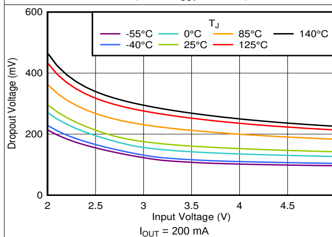
图 35. Dropout vs V_{IN} and Temperature
