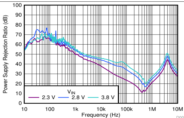
图 45. PSRR vs Frequency and V_{IN}
