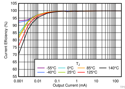
图 63. Current Efficiency vs I_{OUT} and Temperature
