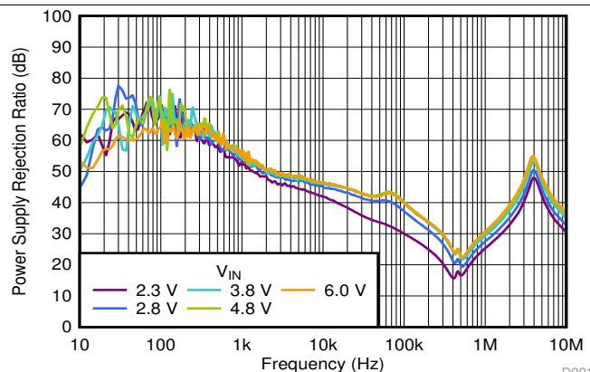
图 46. PSRR vs Frequency and V_{IN}
