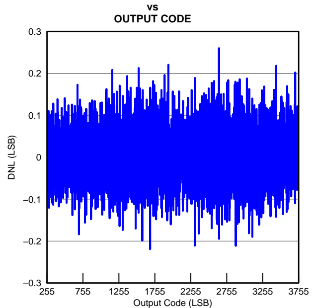
Figure 7-16. DNL Plot
