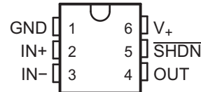
TLV341 DRL Package 6-Pin SOT Top View
