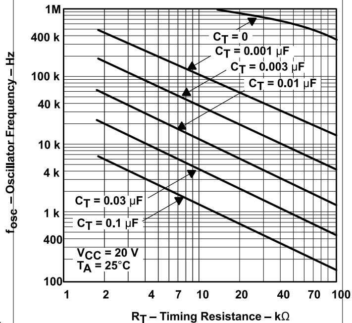
图 7-2. Oscillator Frequency vs Timing Resistance
