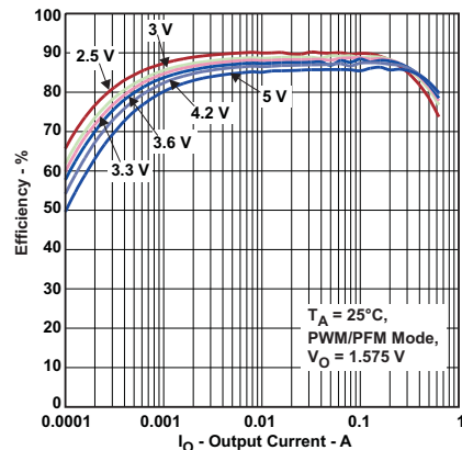
Figure 4. Efficiency DCDC2 (VO = 1.575 V) vs Load Current / PFM Mode
