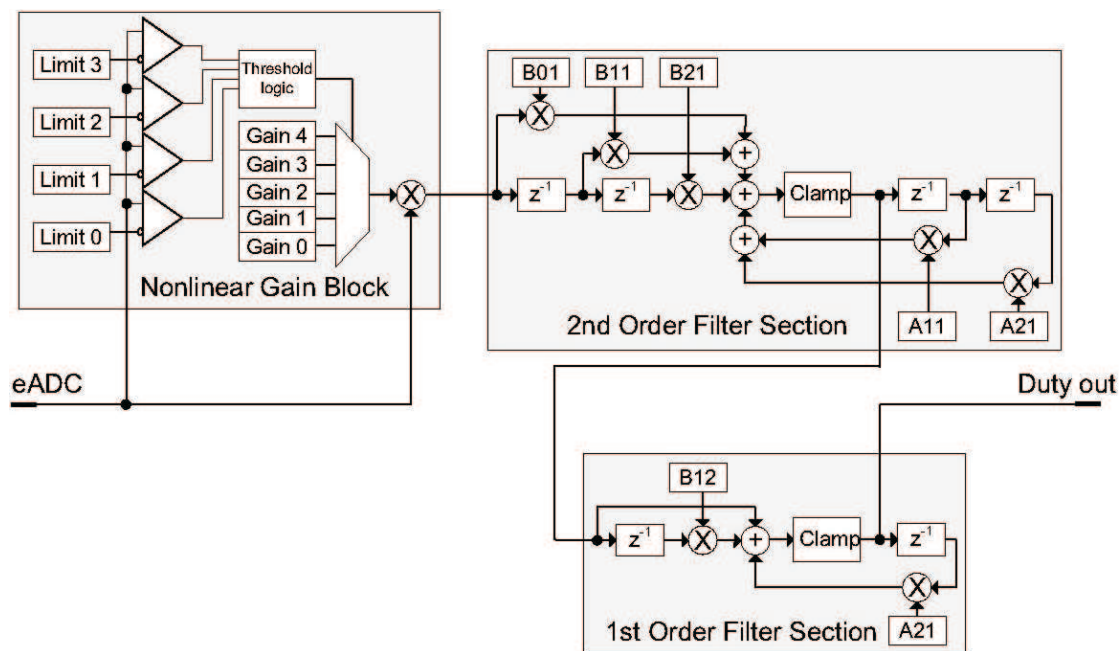
Figure 11. Digital Compensation
