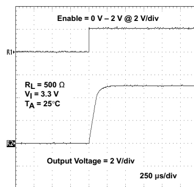
Figure 28. Start-Up Timing
