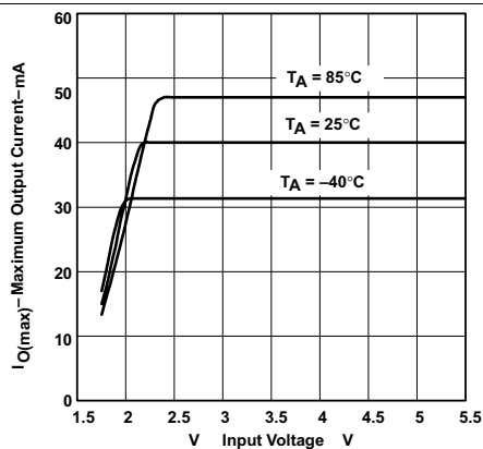
Figure 25. TPS60242
