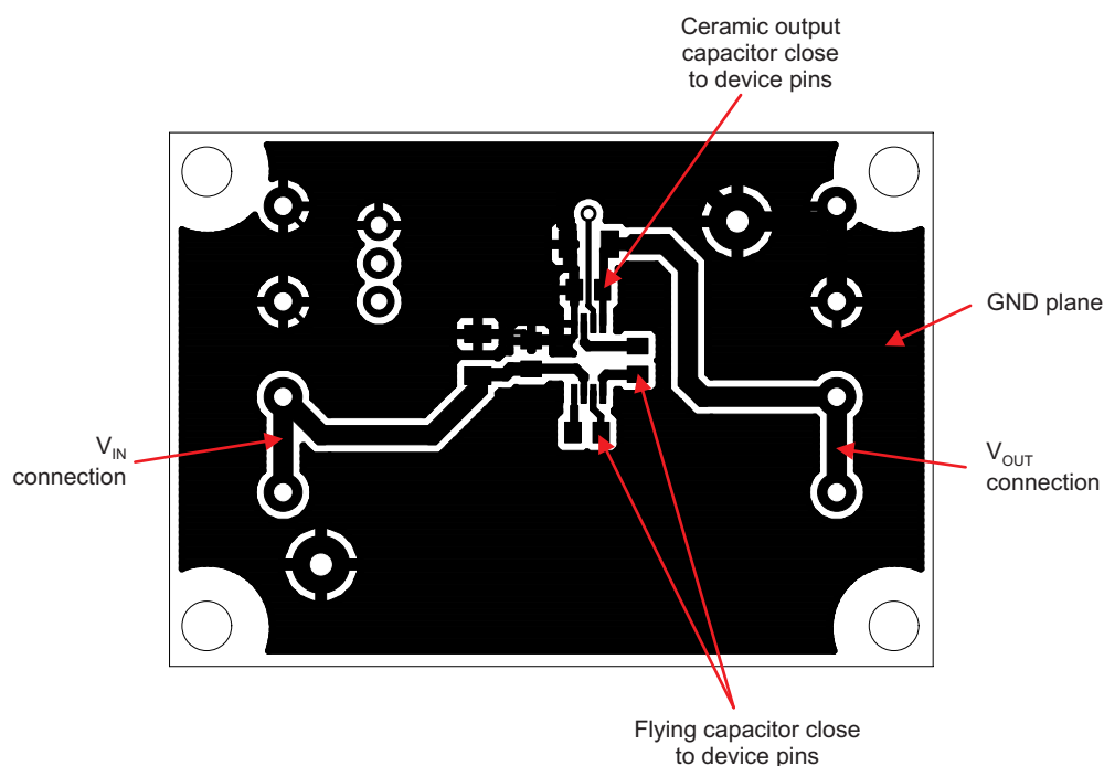
Figure 33. Top Layer
