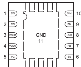
Pin Functions
