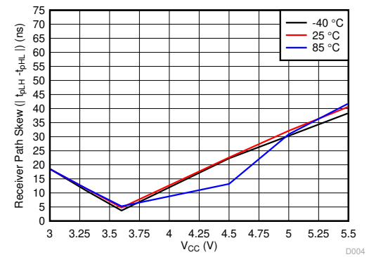
D004_rx_skew.grf
