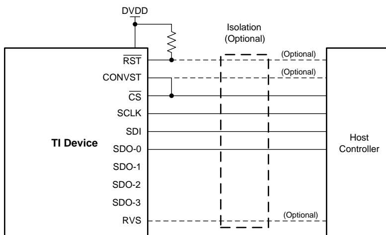
Figure 86. SPI Interface, Minimum Pins
