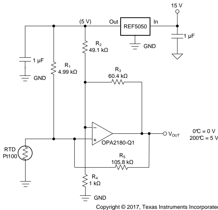
图 34. RTD Amplifier with Linearization
