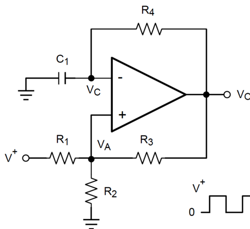
图 44. Square-Wave Oscillator
