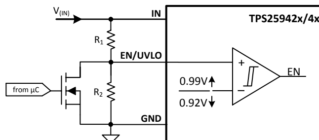
Figure 54. Shutdown Control
