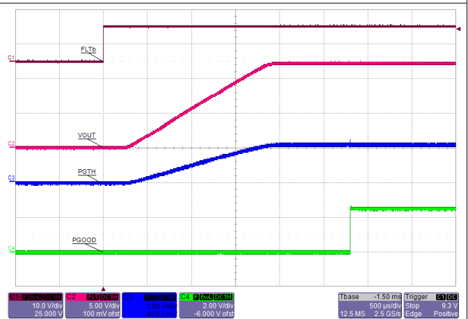
Figure 72. Power Good Response During Turnon
