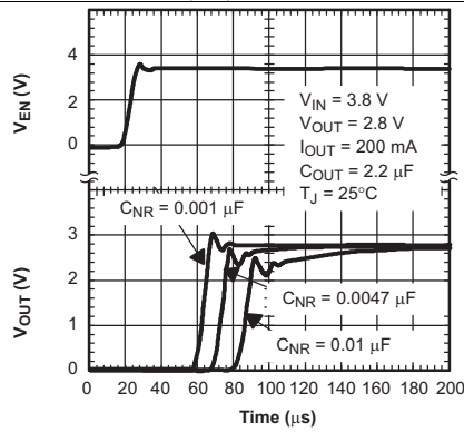
Figure 13. TPS79328 Output Voltage, Enable Voltage vs Time (Start-Up)
