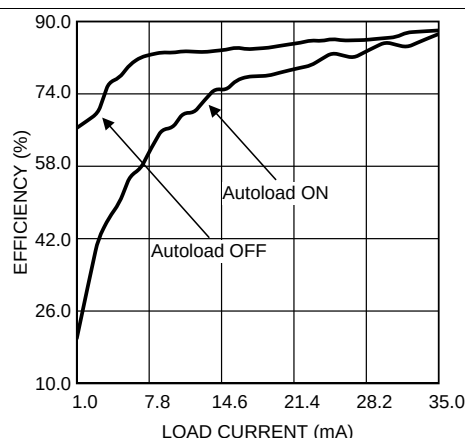
Figure 31. Efficiency at Low Load vs Autoload
