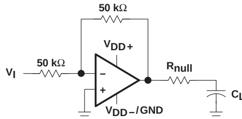
Figure 60. Series-Resistance Circuit
