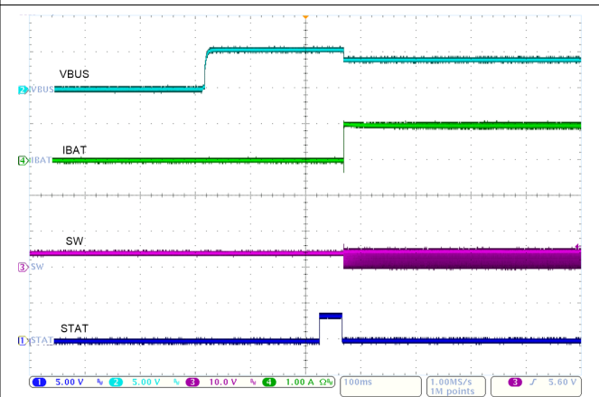
VBUS = 5 V Adaptor Current Limit: 1A ICHG = 2A VBAT = 3.5V
