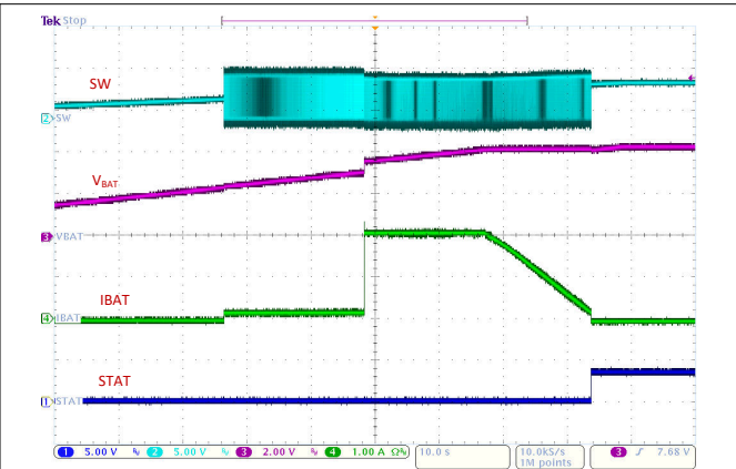
VBUS = 5 V VBAT = 1.5V - 4.2V ICHG = 2 A VBATREG = 4.2V
