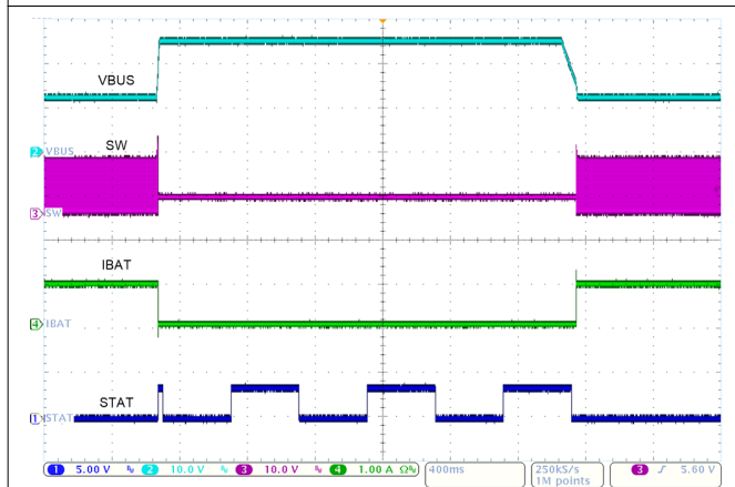
VBUS = 12V -25V -12V VBAT = 3.8V ICHG = 1A
