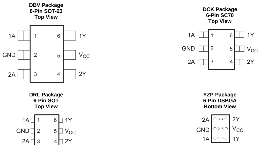
Pin Functions (1)
