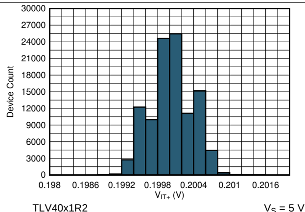
图 10. Positive Threshold Histogram
