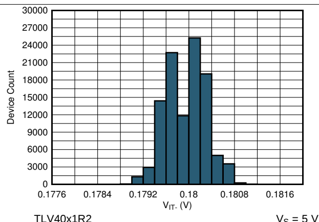
图 12. Negative Threshold Histogram
