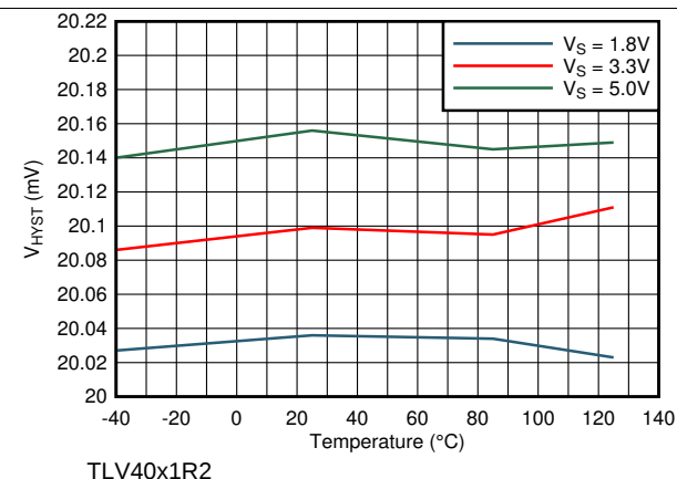
图 13. Hysteresis vs Temperature
