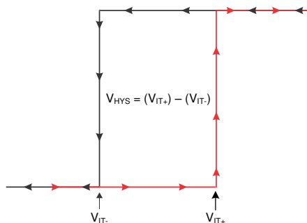
图 38. Transfer Curve
