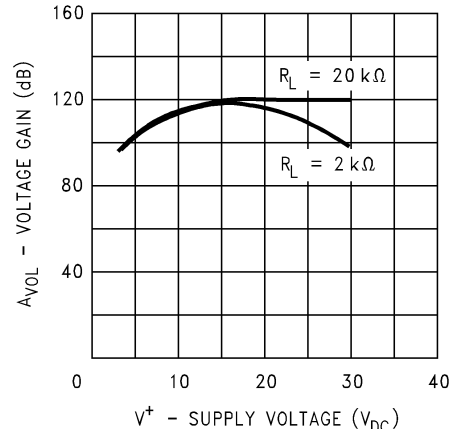
Figure 4. Voltage Gain
