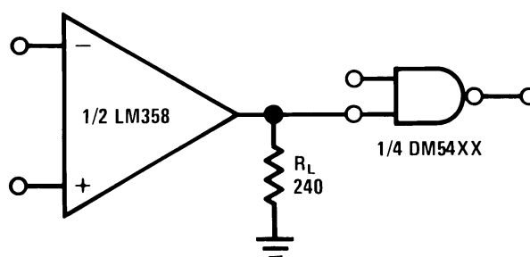
Figure 24. Driving TTL
