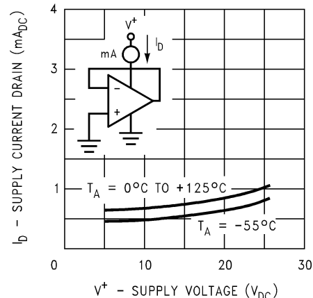
Figure 3. Supply Current
