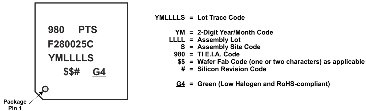
图 10-3. Package Symbolization for PT Package
