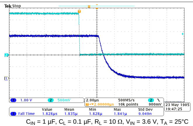
Figure 21. Turn-Off Response
