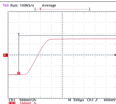
Figure 36. Turn-On Response
