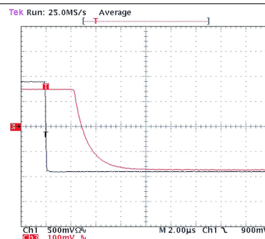
Figure 37. Turn-Off Response
