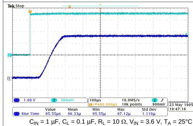
Figure 20. Turn-On Response
