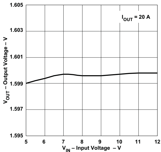
Figure 2. Line Regulation
