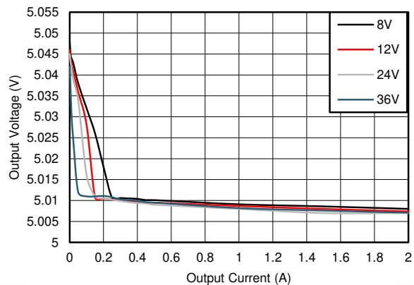
图 9-19. Line and Load Regulation
