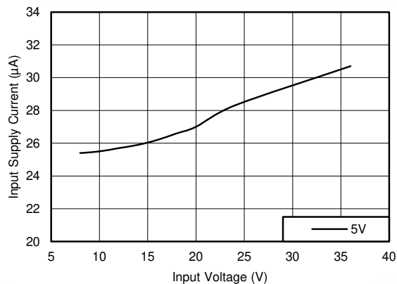
图 9-20. Input Supply Current
