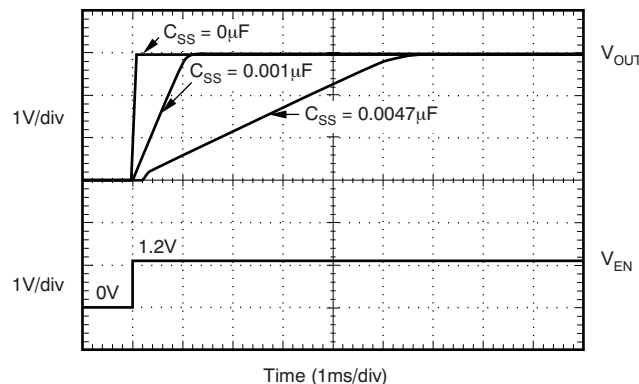
Figure 31. Turnon Response
