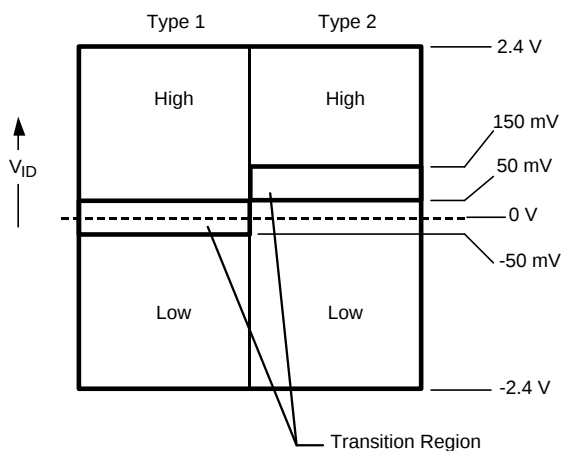
Figure 3. M-LVDS Receiver Input Thresholds
