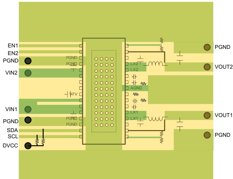
Figure 33. TPS563900 Layout on 2-layer PCB
