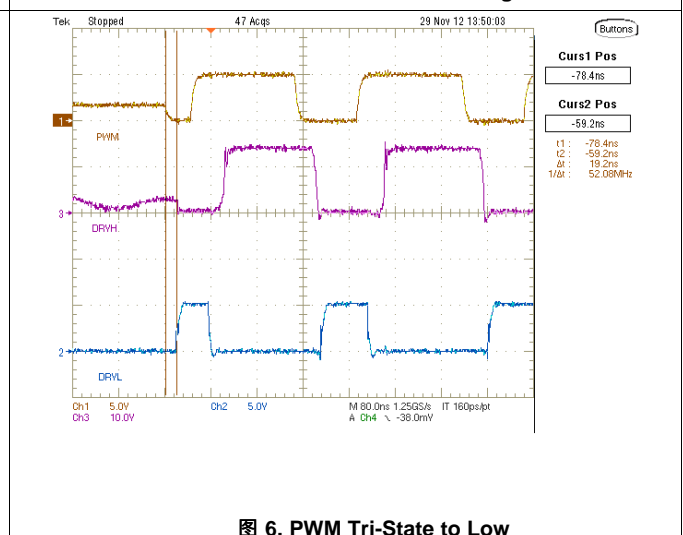
图 6. PWM Tri-State to Low
