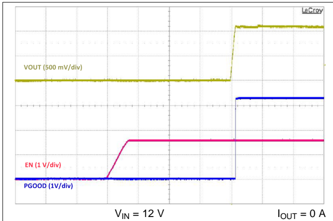
Figure 21. Enable Turn-on
