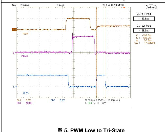
图 5. PWM Low to Tri-State
