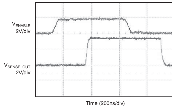
图 17. Enable Power On and Power Off Delay (TPS3895P)
