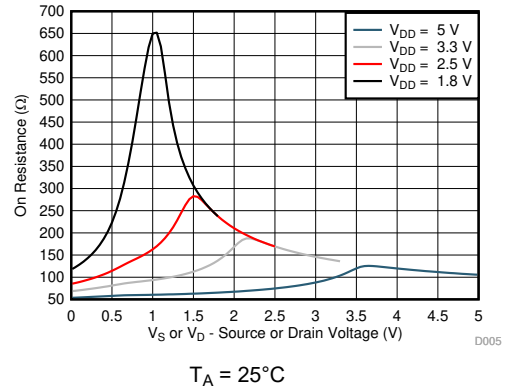
图 7-4. On-Resistance vs Source or Drain Voltage
