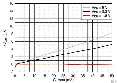
图 7-13. Injection Current vs Maximum Output Voltage shift
