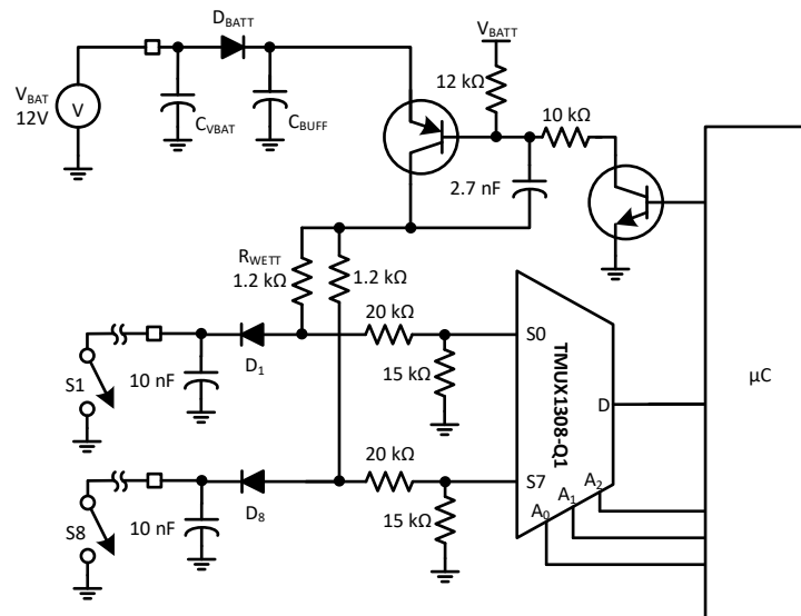
图 9-2. Detailed BCM Application
