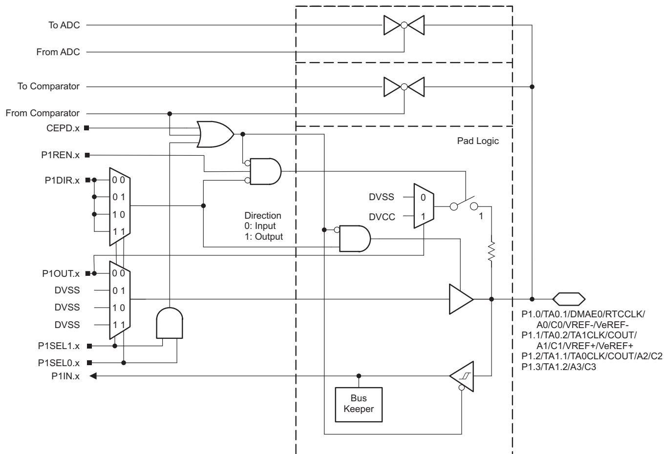
图 6-3. Port P1 (P1.0 to P1.3) Diagram
