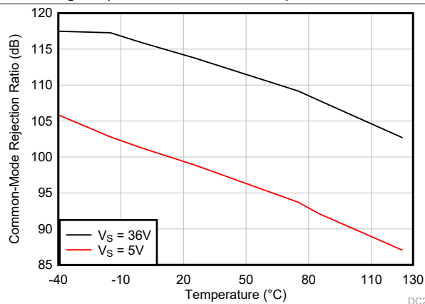
图 14. Common-Mode Rejection Ratio vs Temperature (dB)
