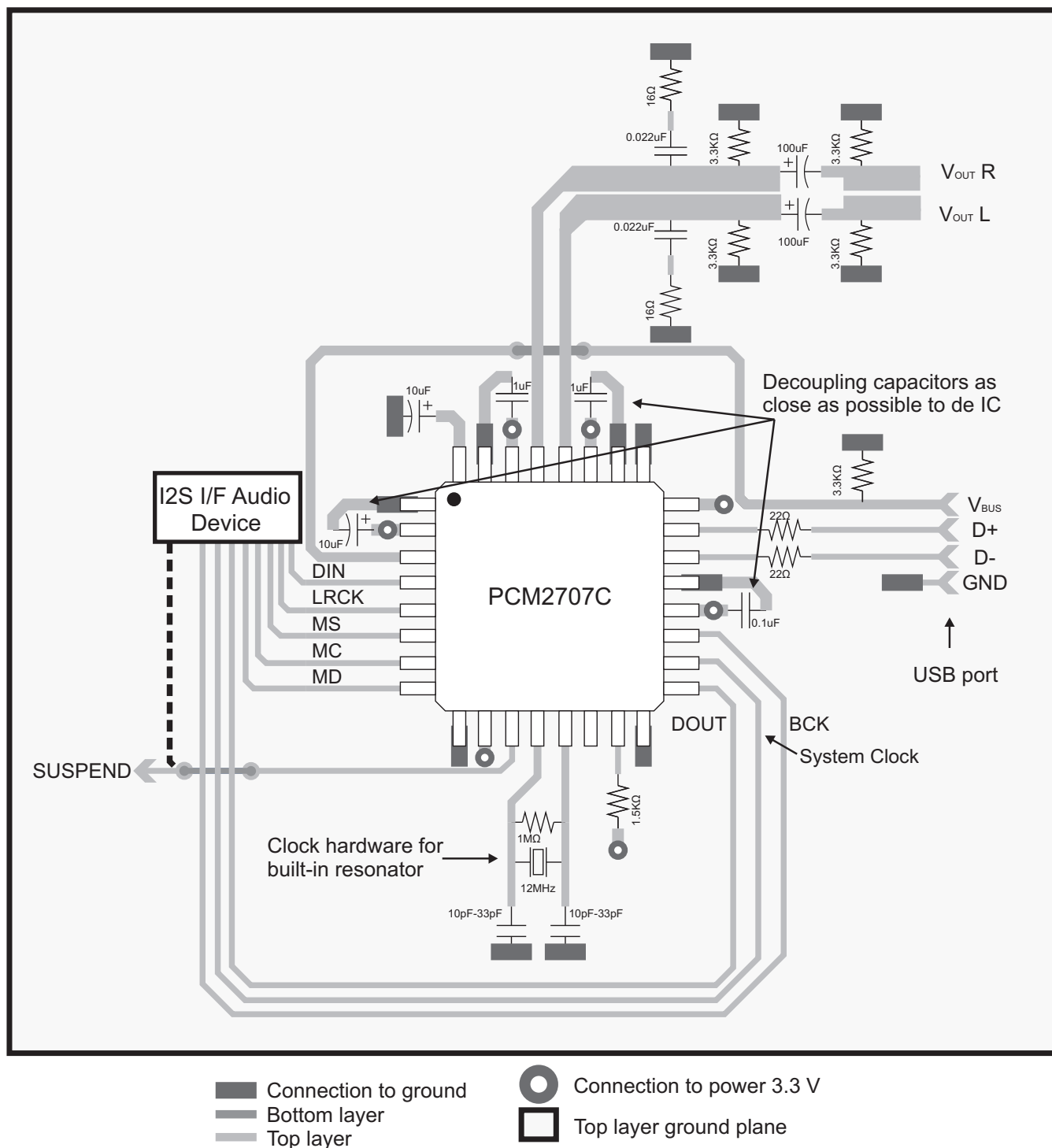
Figure 40. Layout Example 3
