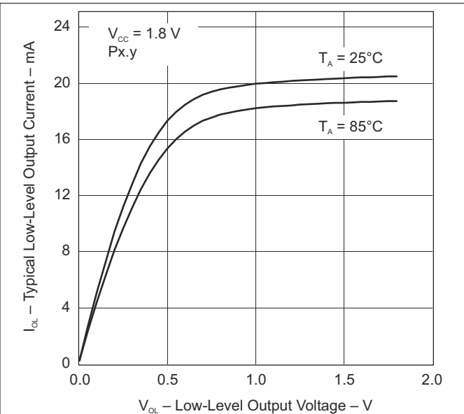
Figure 7-8. Typical Low-Level Output Current vs Low-Level Output Voltage
