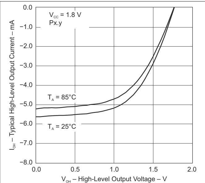
Figure 7-6. Typical High-Level Output Current vs High-Level Output Voltage
