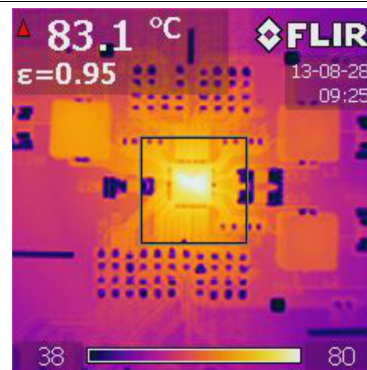
Figure 69. Thermal Signature of TPS65261EVM
