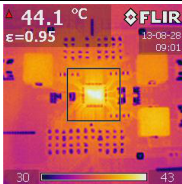
Figure 68. Thermal Signature of TPS65261EVM
