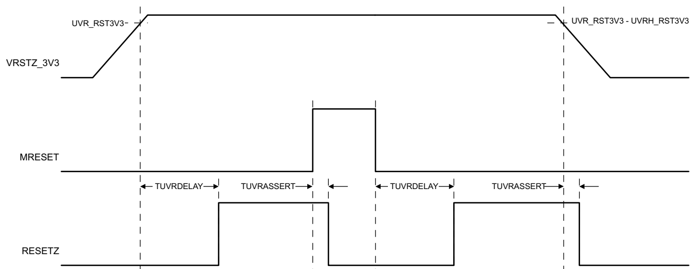
图 8-1. RESETZ Assertion Timing
