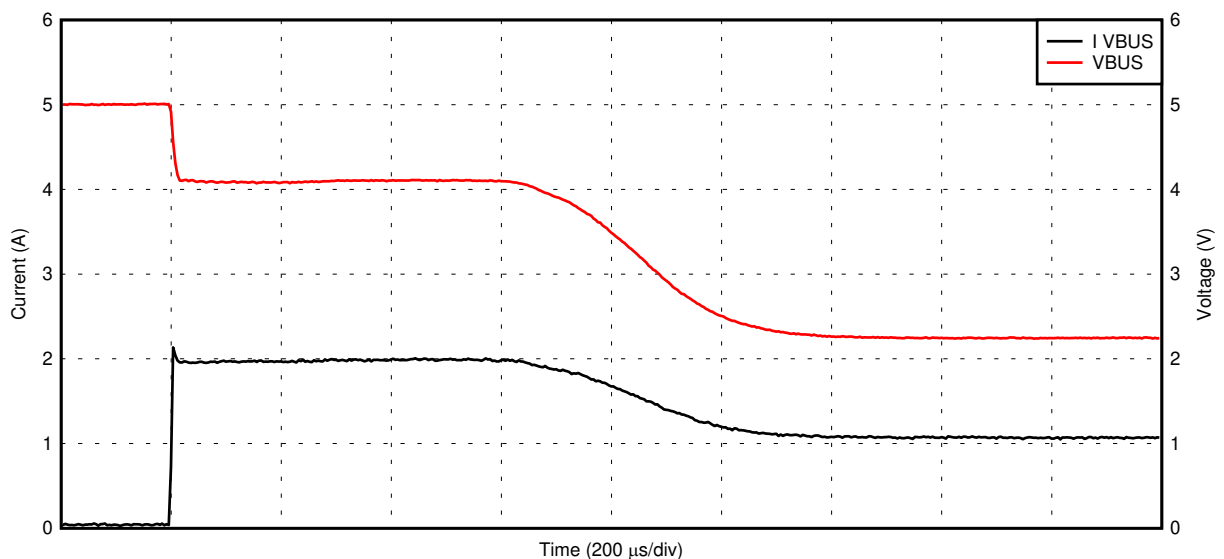
图 9-15. PP_5V0 Current Limit with a Soft Short (2 \Omega )
