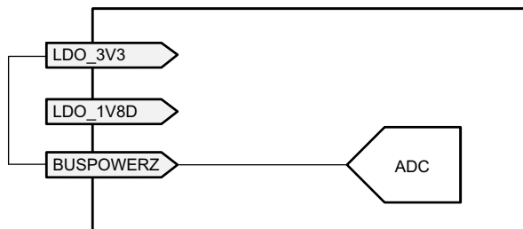
图 9-22. BUSPOWERZ Configured to Disable Power from VBUS
