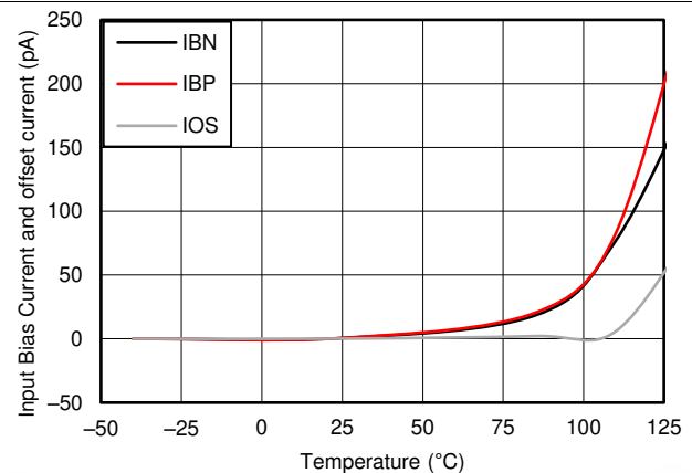
图 6. Input Bias Current vs Temperature
