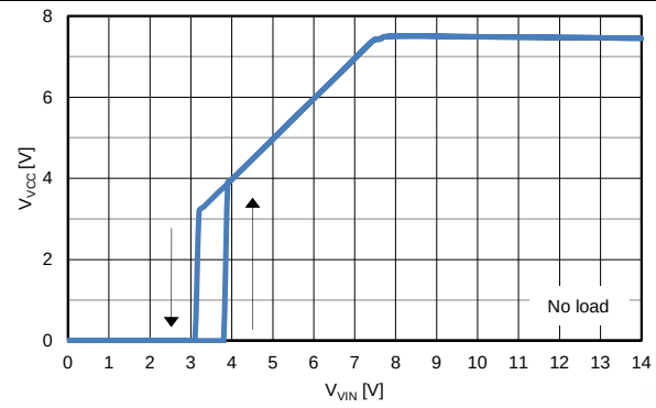
Figure 8. V_{CC} vs V_{IN}
