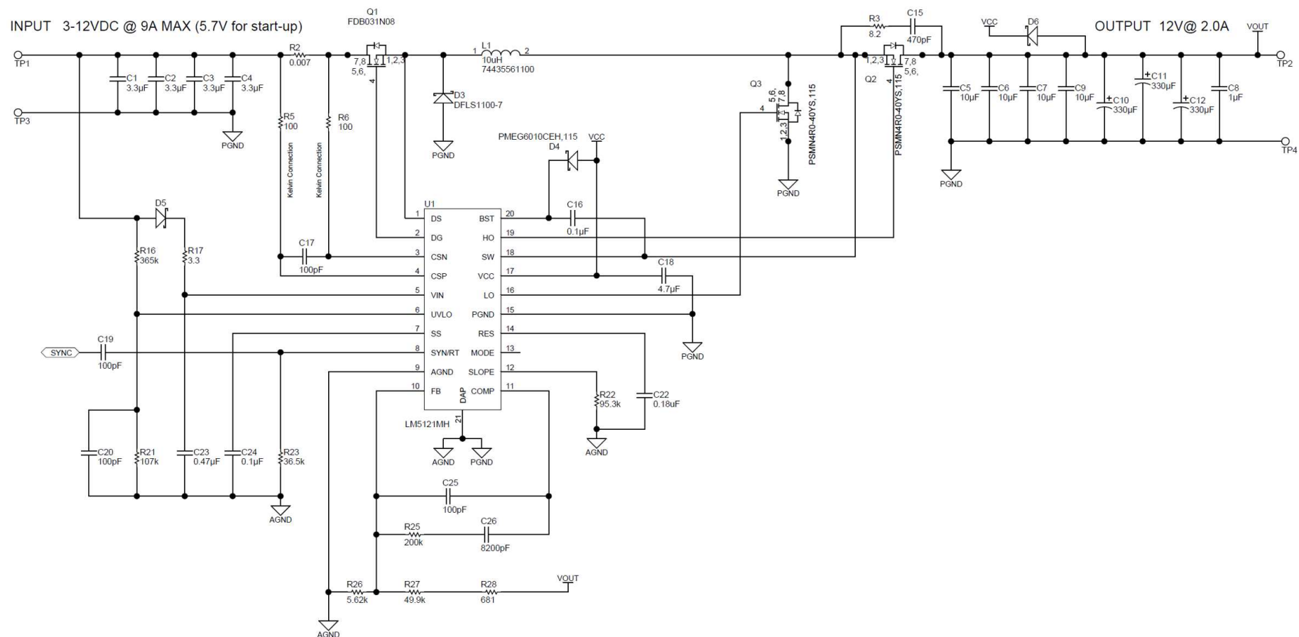
Figure 39. Schematic
