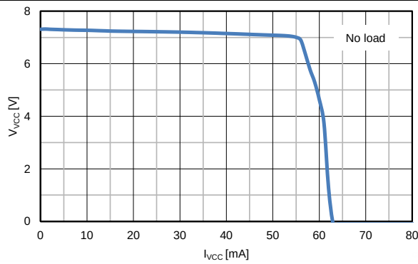
Figure 7. V_{CC} vs I_{CC}
