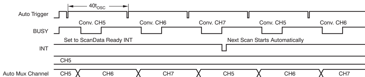
Figure 24. Mode 6 Timing
