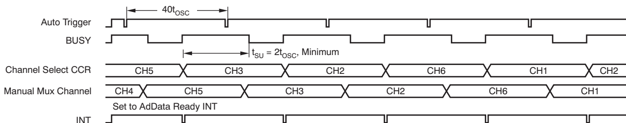
Figure 25. Mode 4 Timing
