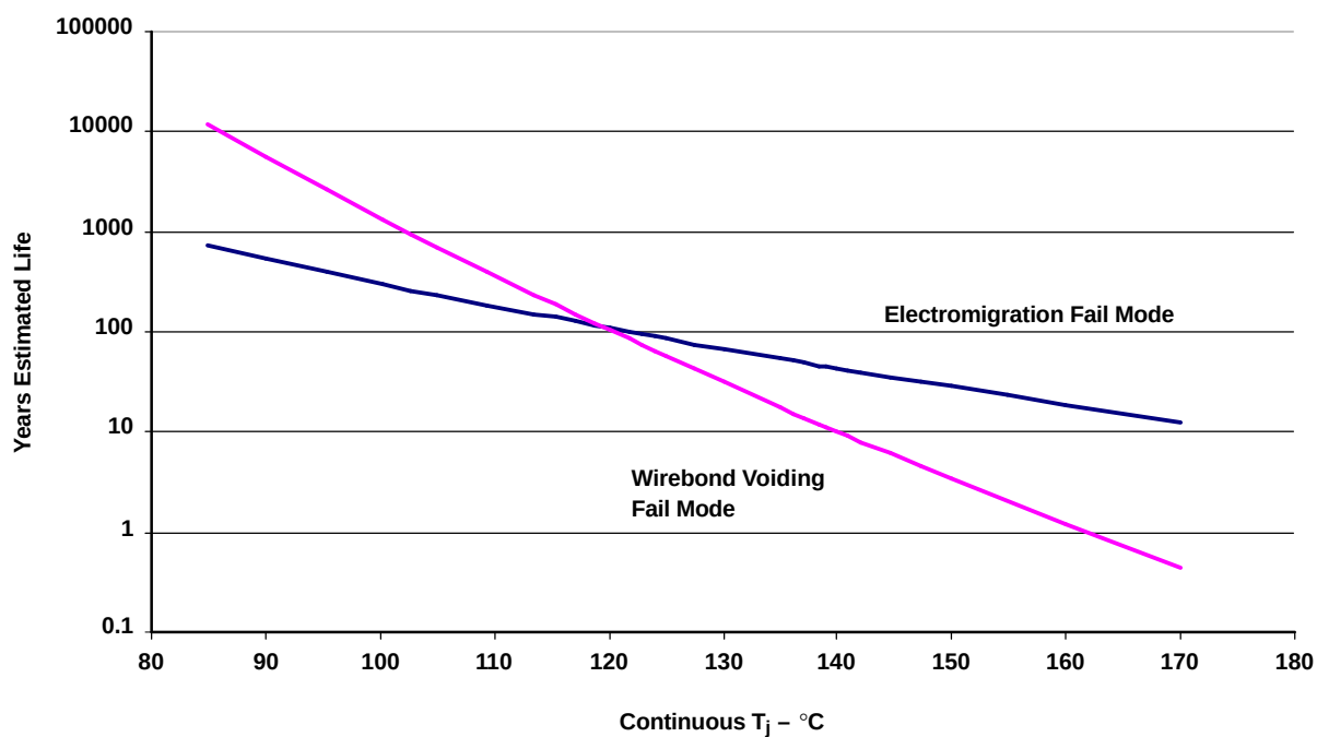
Figure 2. CABT16373AMDLEP Operating Life Derating Chart
