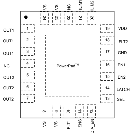
图 6-3. RHF Package 24-Pin QFN Top View Version D
