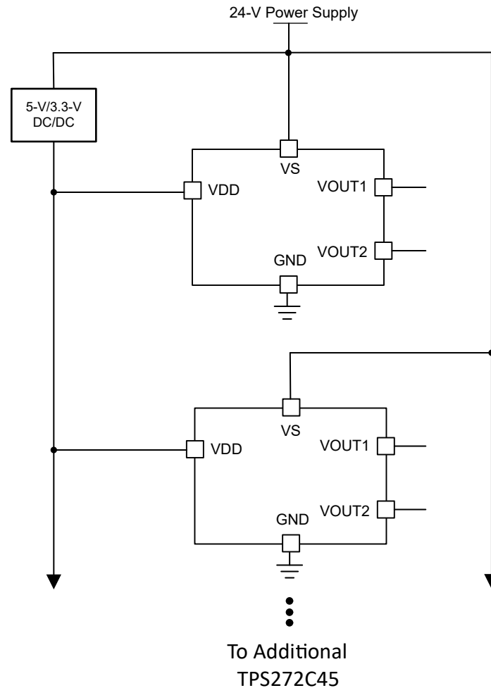
图 9-6. Secondary Low Voltage Supply Schematic
