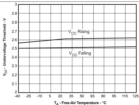
Figure 8. V_{CC} Undervoltage Threshold vs Free-Air Temperature
