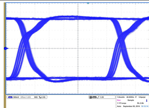
Figure 25. ISO7242M Eye Diagram at 150 Mbps, 3.3 V and 25°C
