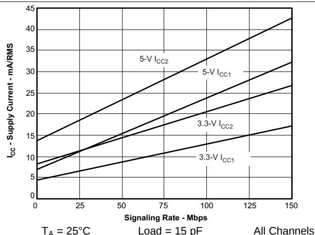
Figure 4. ISO7241C/M RMS Supply Current vs Signaling Rate
