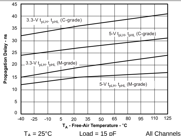
Figure 6. Propagation Delay vs Free-Air Temperature
