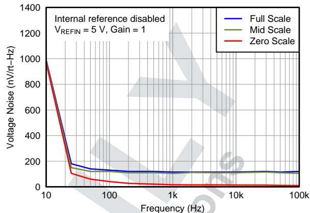
图 45. DAC Output Noise Density vs Frequency
