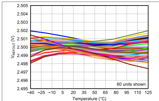
图 2. Internal Reference Voltage vs Temperature
